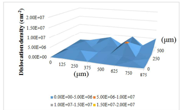
Non-Core GaN Ave: 8.7E+5(cm -2 )
