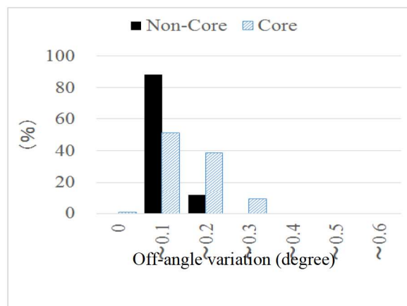
Fig. 7. Off-angle variation histogram for GaN substrate.
