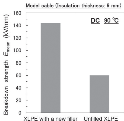
Fig. 10. DC breakdown strength of new XLPE cable with a new filler (DC-XLPE) and unfilled XLPE cable (AC-XLPE) (17)
