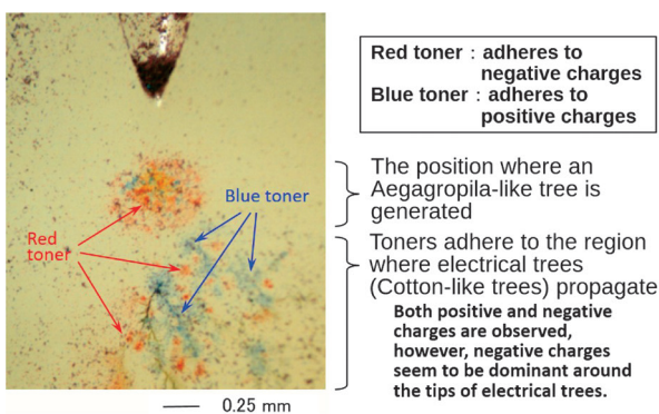
Photo 4. Dust figure pattern of treeing sample after AC 18 kV × 30 min. & AC 10 kV × 2 h voltage application (4)
