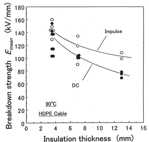
Fig. 4. Insulation thickness dependence of breakdown strengths of HDPE cables (13)
