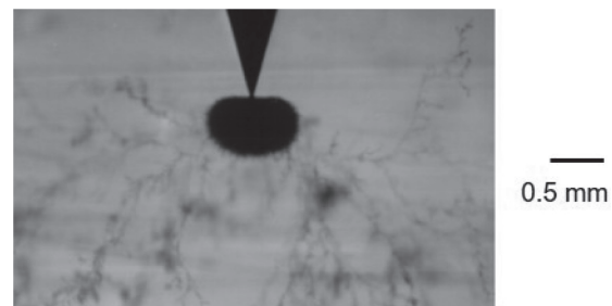
Photo 3. Feature of electrical trees (an Aegagropila-like tree & Cotton-like trees) after AC 18 kV \times 30 min. & AC 10 kV \times 2 h voltage application (4)
