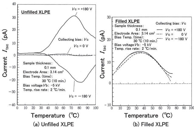
Fig. 7. TSC spectra of unfilled and filled XLPEs (15)
