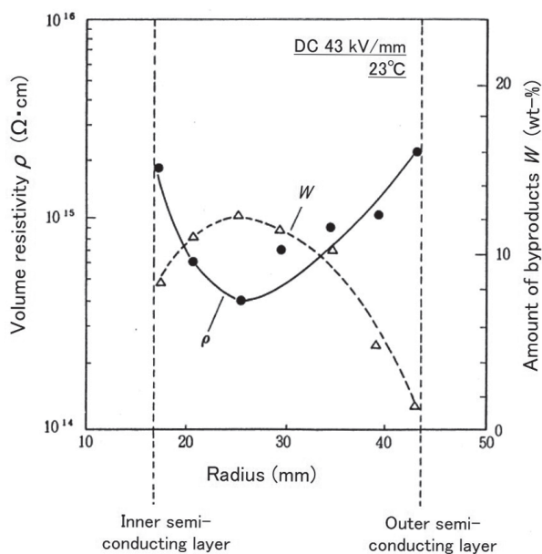
Fig. 2. Distribution of volume resistivity \rho and amount of peroxide byproducts W in 275 kV XLPE cable (27 mm-t, 600 mm 2 ) in the radial direction of the insulator (12)
