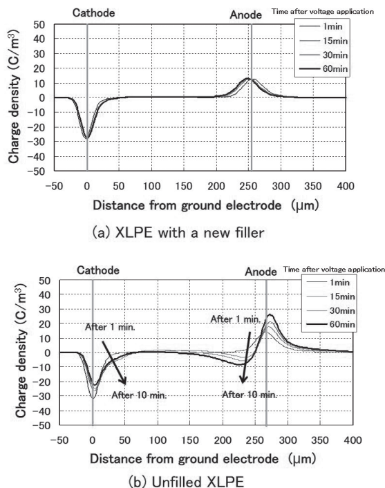
Fig. 9. Space charge distribution of XLPE with a new filler (DC-XLPE) and unfilled XLPE (AC-XLPE) (18)
