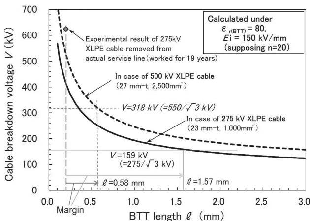
Fig. 14. Relationship between BTT length and breakdown voltage of 275 kV & 500 kV XLPE cables (23)
