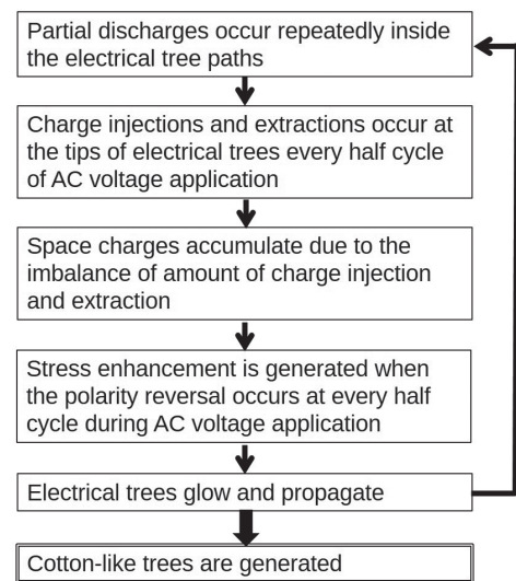
Fig. 1. Schematic representation of generation mechanism of Cotton-like trees (4)
