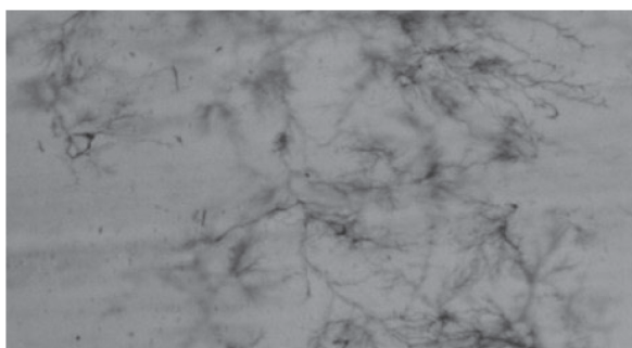
Photo 2. Electrical trees in random directions (named “Cotton-like trees”) observed near a breakdown path in XLPE base insulation of a product (1)
