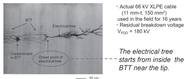
Photo 5. Example of electrical tree starting from a BTT in an actual 66 kV XLPE cable (22)
