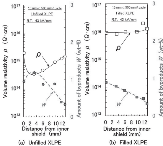
Fig. 6. Difference between filled and unfilled XLPE cables in volume resistivity \rho and amount of peroxide byproducts W in the radial direction of the insulator (15)
