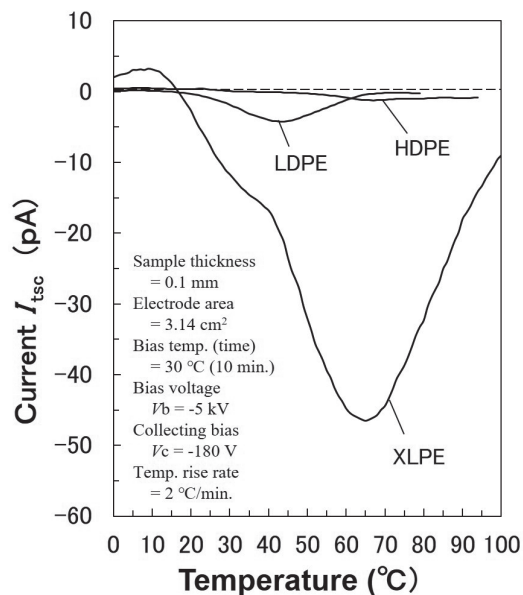
Fig. 3. TSC spectra of XLPE, LDPE and HDPE (13)
