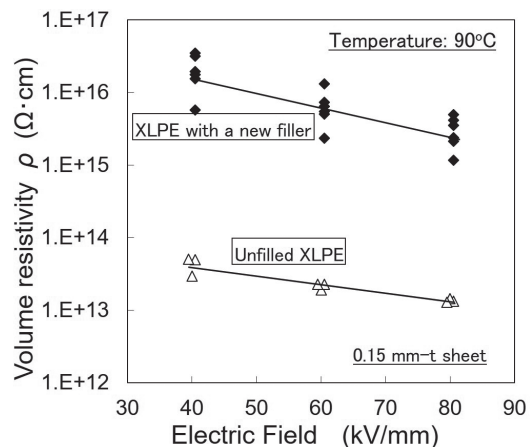
Fig. 8. Electric field dependence of volume resistivity of XLPE with a new filler (DC-XLPE) and unfilled XLPE (AC-XLPE) (17)
