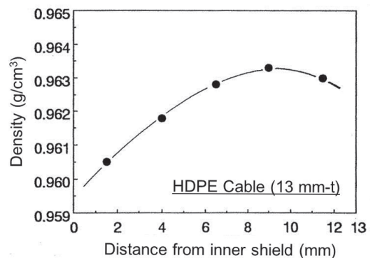
Fig. 5. Density distribution of HDPE cable insulation (13 mm-t) (13)
