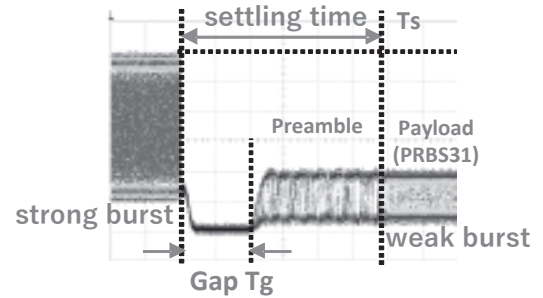
Fig. 6. Input optical signals for bit error ratio measurement
