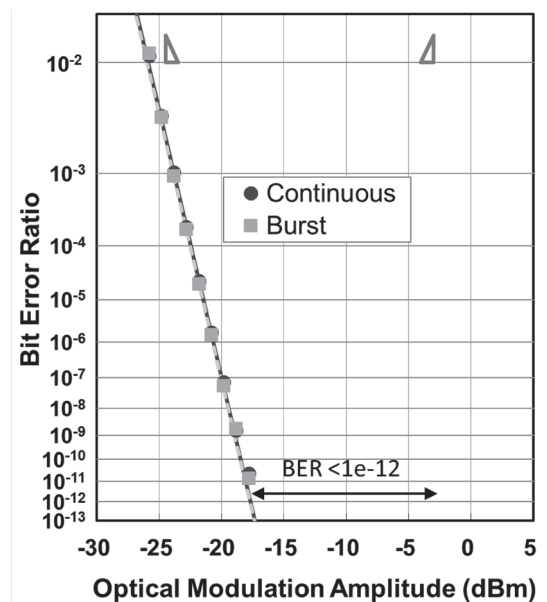
Fig. 7. 25.78 Gbit/s Bit Error Ratio results
