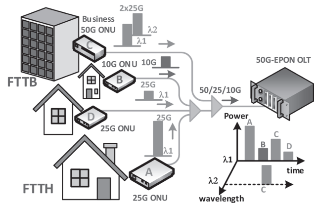
Fig. 1. 50G-EPON system overview and upstream transmission
