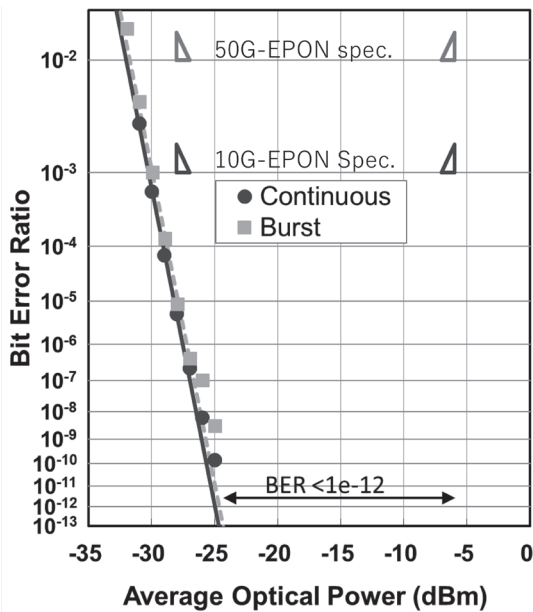
Fig. 8. 10.31 Gbit/s Bit Error Ratio results
