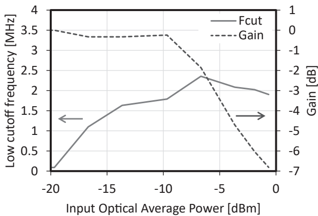
Fig. 4. Dependence of low-pass cutoff frequency Z_{T(O-E)} on optical input power
