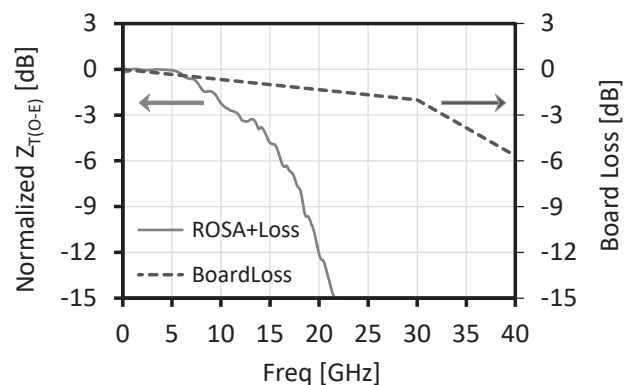
Fig. 3. High-frequency response of optoelectronic conversion gain ( Z_{T(O-E)} )
