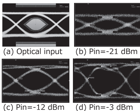
Fig. 5. 25.78 Gbit/s optical input and electrical output waveforms
