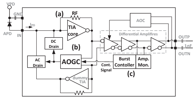
Fig. 2. Block diagram of 25.78 Gbit/s BM-TIA
