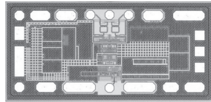
Photo 2. A photo of BM-TIA IC chip
