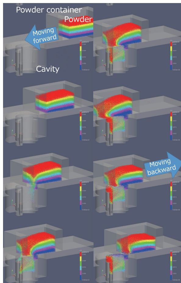
Fig. 5. Powder feeding simulation results. Coloring of particles indicates their elevations observed before filling (11)
