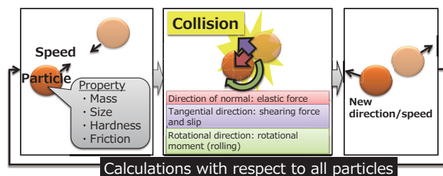
Fig. 1. DEM-based simulation algorithm for powder particle behavior (11)
