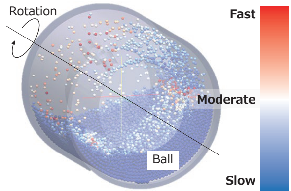
Fig. 2. Ball mill simulation; balls are colored according to speeds (11)
