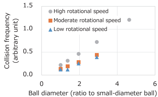
Fig. 4. Relationship between the number of collisions and rotational speed (11)
