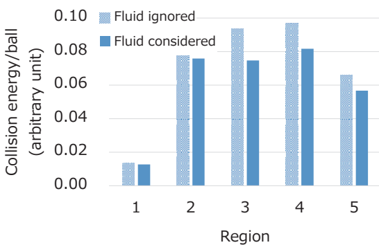
Fig. 3. Ball collision energy (11)
