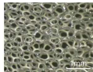
Heatproof and anticorrosion Celmet
