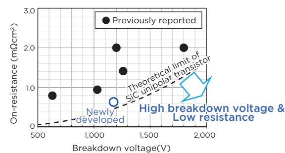
Structure and on-resistance of next generation VMOSFET
