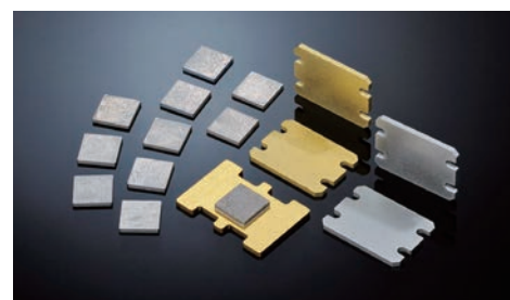
Ag-Dia heatspreader
