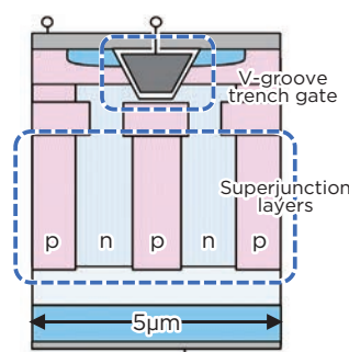
Structure and on-resistance of next generation VMOSFET
