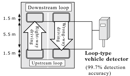
Fig. 2. Example of loop-type vehicle detector configuration
