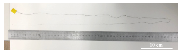
Photo 2. CNT yarn resin composite material (1 m long)
