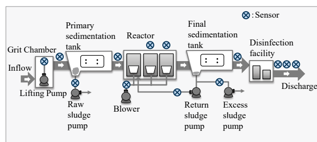
Fig.1. Schematic diagram of sewage treatment plant
