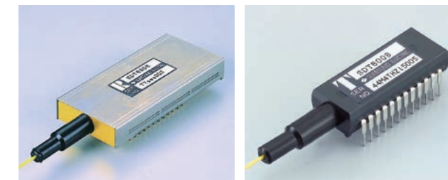
2.5 Gbps optical link
