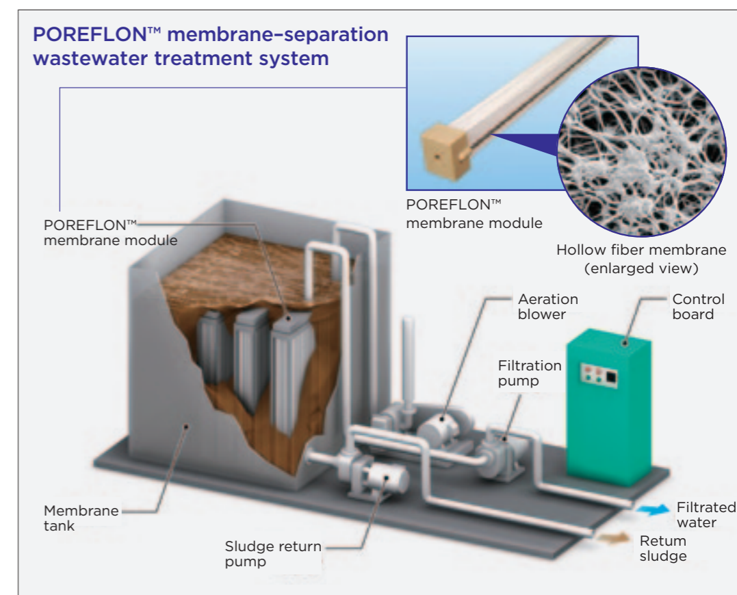
Wastewater treatment system installed in the Kisa Plant
