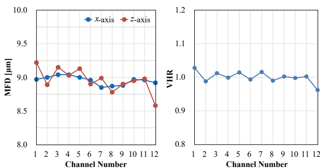
Fig. 8. NFP measurement result at 1.31μm wavelength (a) MFD in the X and Z direction (b) VHR of each core
