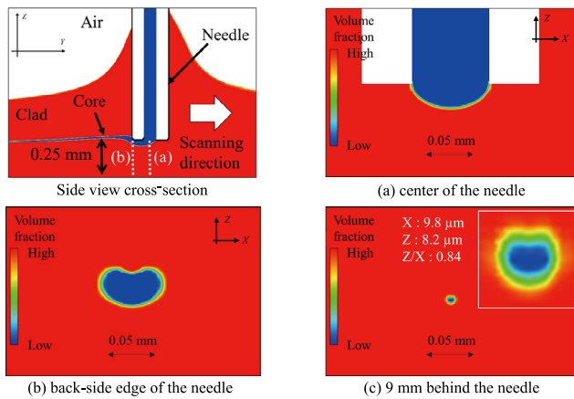
Fig. 6. Cross section perpendicular to the needle scanning direction (a) Center of the needle ( Y = 0 mm) (b) Back-side edge of the needle ( Y = 0.115 mm) (c) 9 mm behind the needle ( Y = 9.115 mm) (15)
