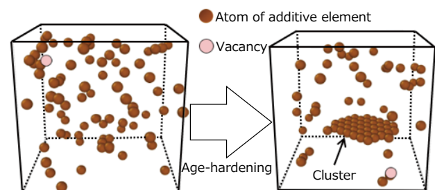
Fig. 7. Age-hardening calculation of aluminum wire (aluminum atoms are not shown)
