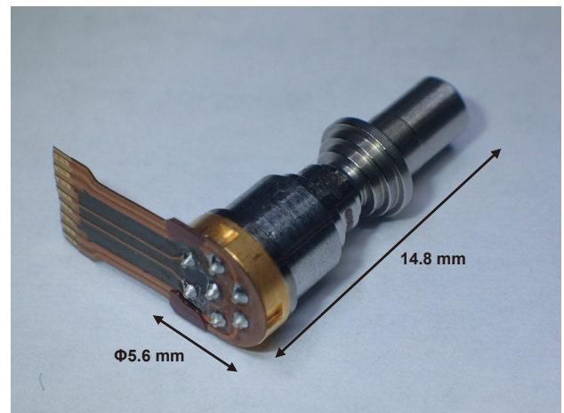
Photo 2. Optical receiver
