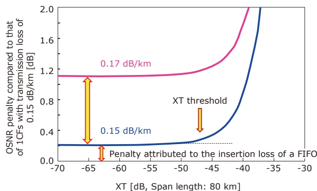
Fig. 6. OSNR penalty of 2CF compared to that of 1CF
