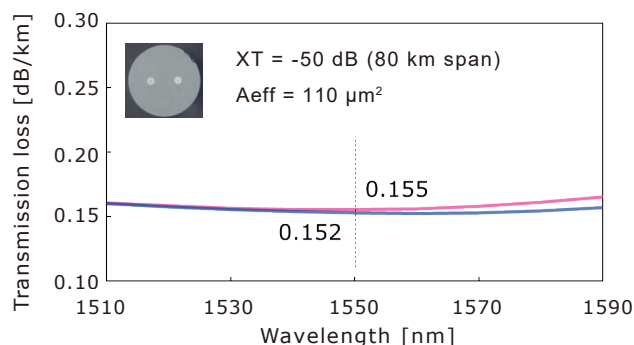
Fig. 7. Wavelength characteristics of 2CF transmission loss
