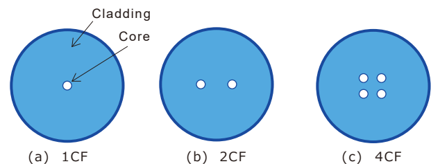
Fig. 4. Schematic cross section of a multi-core fiber
