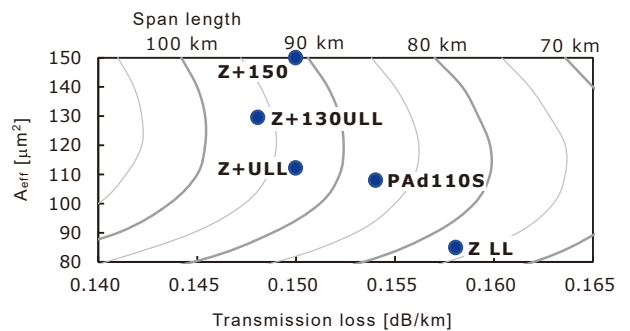
Fig. 3. Span length as a function of A_{\text{eff}} and transmission loss (Transmission distance: 7,000 km, 48 cores, Cable transmission capacity: 0.5 Pb/s)
